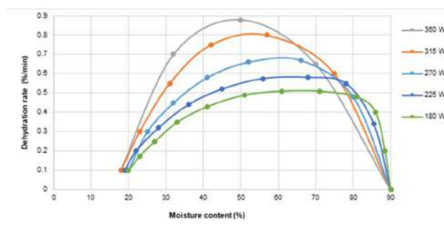
Fig. 5. Dehydration kinetics curves of pears dried by the combined method
