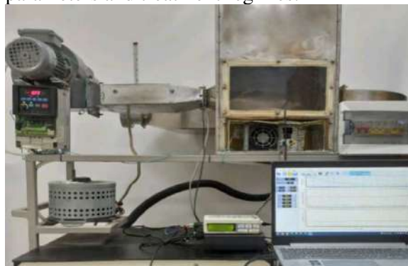
Fig. 1. The experimental installation developed for the dehydration of fruits with the application of the combined treatment method
