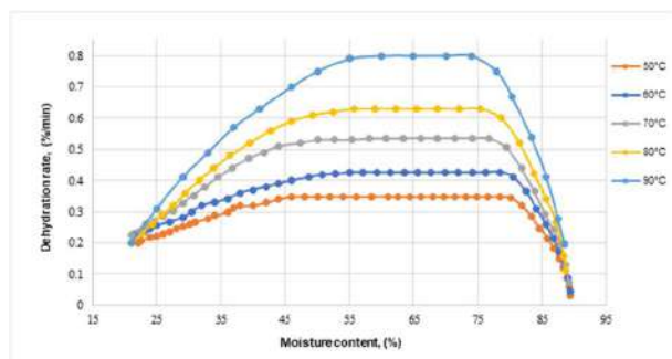
Fig. 4. Dehydration kinetics curves of pears dried by the traditional method
