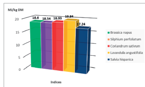
Figure 3. Gross calorific value of biomass
