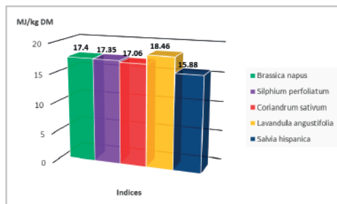
Figure 4. Net calorific value of biomass
