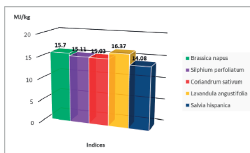
Figure 5. Net calorific value of pellets
