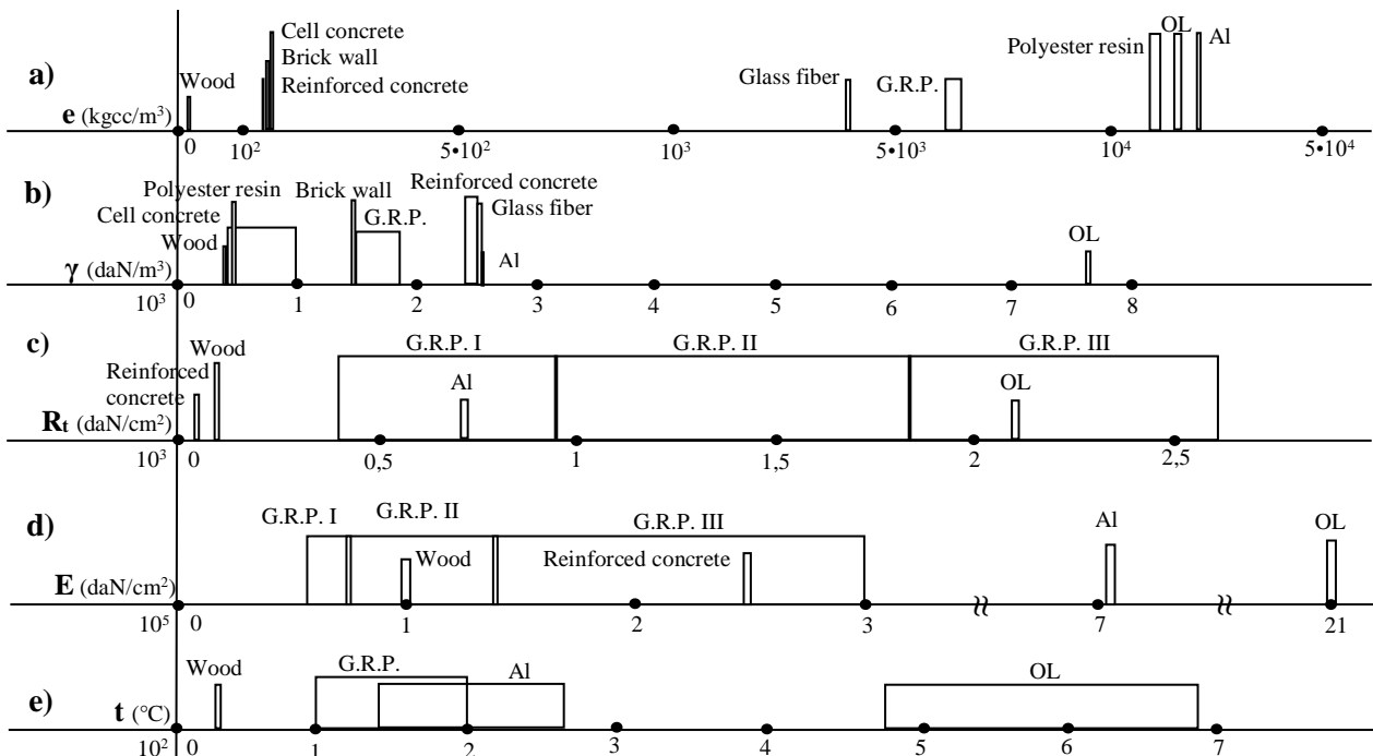
Figure 4. Place of prime materials and composite materials in comparison with traditional materials, function of some physical and mechanical characteristics.
