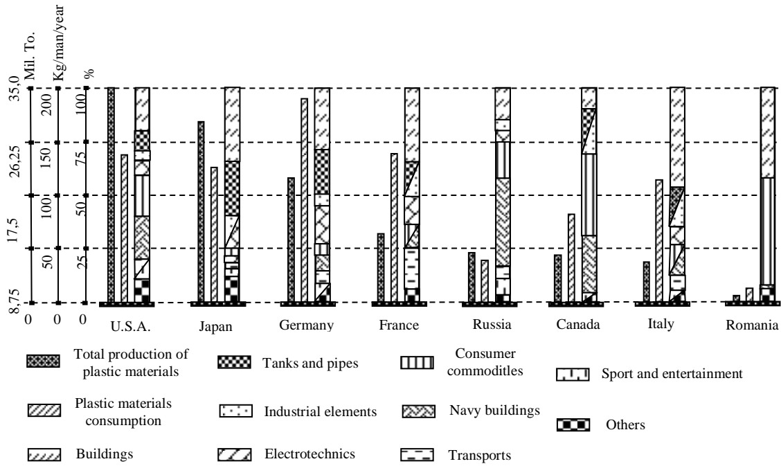
Figure 3. Plastic material production, consumption per man, per year and the weight of their use in different domains and countries.
