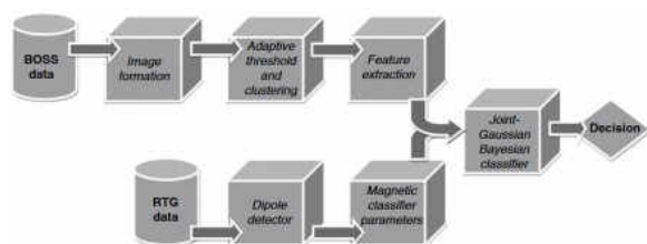
Fig. 5. Acoustic and magnetic sensor fusion system (redrawn from [34]).
