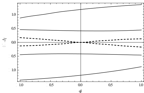
Fig. 2 The energy spectrum of the mixed exciton-plasmon (solid line) and acoustical plasmon (dashed lines) collective elementary excitations of the Bose-Einstein condensed 2D magnetoexcitons with dimensionless wave vector \vec{k} = 0 and filling factor P = 0 .
