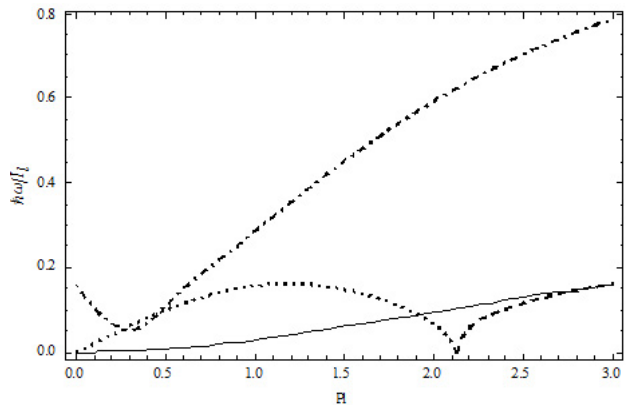
Fig.1 Three branches of the collective elementary excitations: the exciton-type quasi-NG mode with a gap in the point pl = 0 (dash-dotted line); the second-type NG mode describing the optical plasmons(solid line) and the first-type NG mode with absolute instability (dotted line) describing the acoustical plasmons(dashed line).
