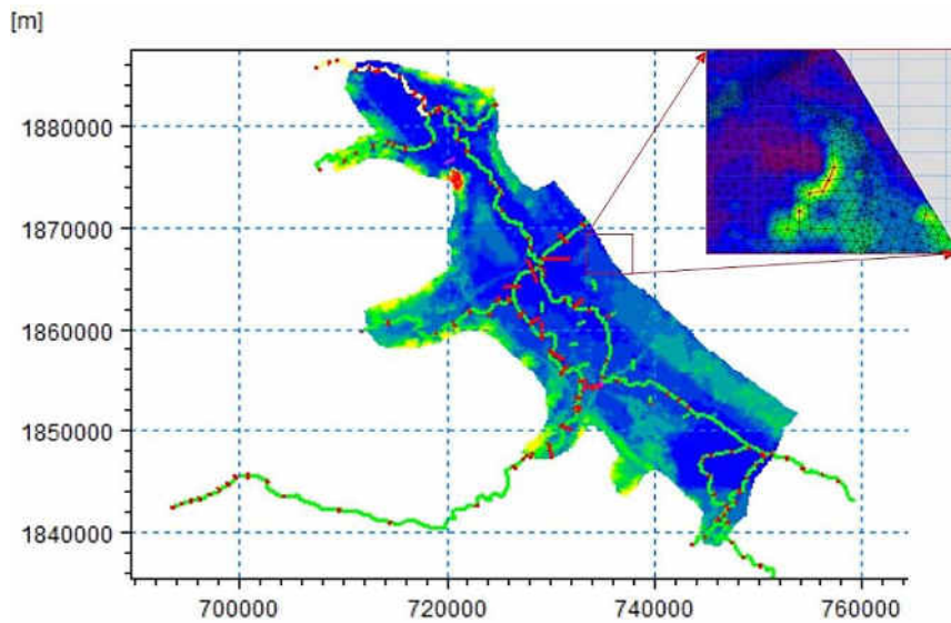
Figure 3. Coupling between 1D and 2D models in the computational domain
