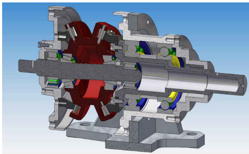
Fig. 4.2. Transmisia precesională cu angrenare de tipul A^B_{CX-CV} ( Z_1 = 26, Z_2 = 27, Z_3 = 22, Z_4 = 21 , \delta_{(1-2)} = \delta_{(3-4)} = 22,5^\circ, \beta_{(1-2)} = 3,5^\circ, \beta_{(3-4)} = 4,78^\circ, \theta = 3,5^\circ, R_m = 46 \text{ mm}, r_2 = 2,9 \text{ mm}, r_3 = 4,38 \text{ mm} ).
