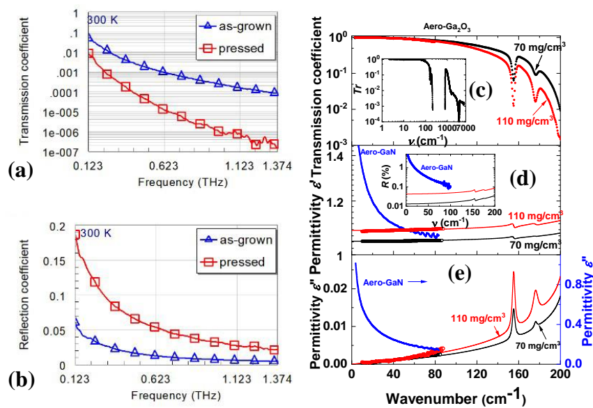
Fig. 12. The measured (a) transmission and (b) reflection coefficients and their temperature dependency of the aero-GaN samples with densities of 0.3 \text{ g/cm}^3 (the “as-grown” sample) and 0.35 \text{ g/cm}^3 (“pressed” sample) [21]; the electrodynamic characterization in the THz region of the aero- Ga_2O_3 with densities of 70 \text{ mg/cm}^3 and 110 \text{ mg/cm}^3 as well as aero-GaN sample with density of 15 \text{ mg/cm}^3 : the transmission coefficient T_r (c), real part \epsilon' (d) and imaginary part \epsilon'' (e) of the dielectric permittivity. The curved marked with dots from figure (d) and (e) represents the THz permittivity data. The insert from figure (c): the measured spectrum of the transmission coefficient at frequencies up to 7000 \text{ cm}^{-1} . The insert from figure (d): the reflectivity coefficient spectrum determined based on the measured spectra of real and imaginary parts of the dielectric permittivity using the standard Fresnel expression [20], [22].
