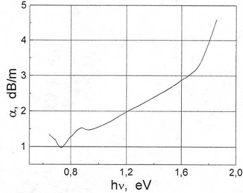
Fig. 2b. Room temperature absorption spectrum in purified \text{As}_2\text{S}_3 glass fibre sample 10 .
