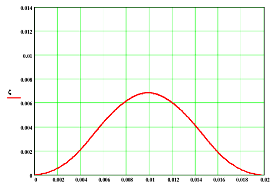
Fig. 3. The influence of the number of teeth on the form of teeth profile.
