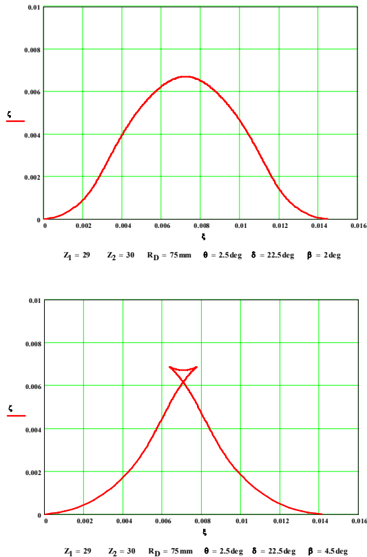
Fig. 5. The influence of the taper angle of the rollers, \beta on the form of teeth profile.
