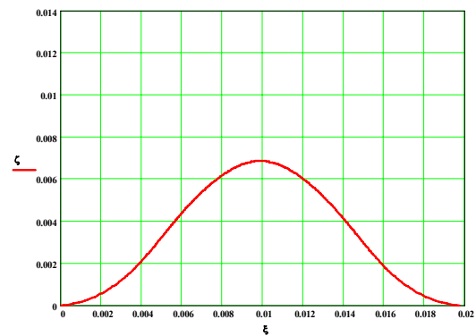
Fig. 3. The influence of the number of teeth on the form of teeth profile.
