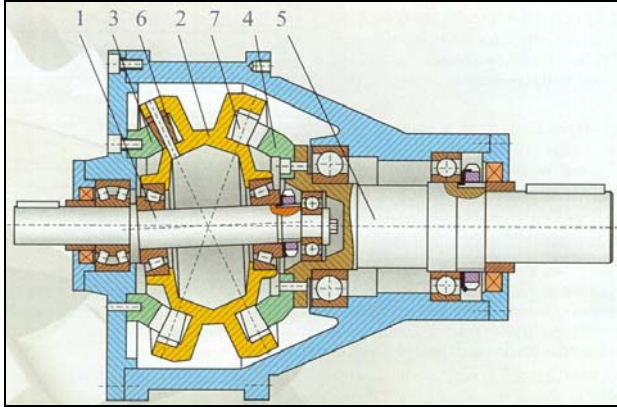
Fig. 1. Diagram of the planetary precessional transmission.
