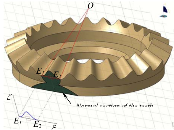
Fig. 6. 3D model of the whole gear.
